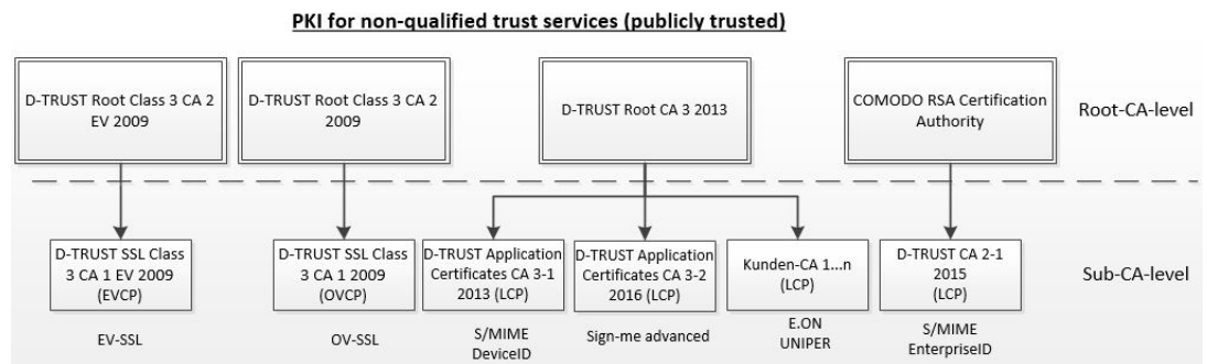
Fig. 2 PKI hierarchy for non-qualified trust services
